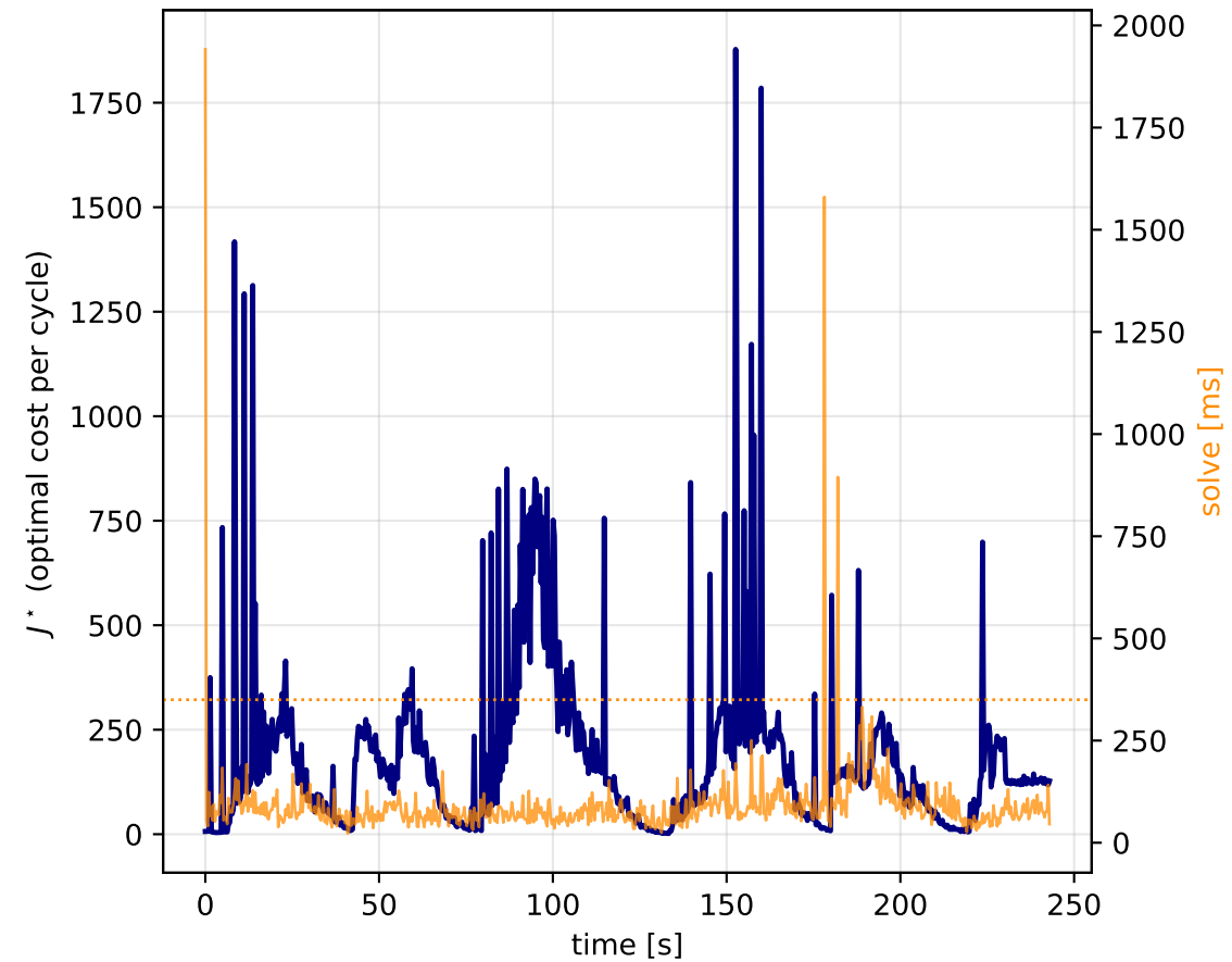
(c) J^* per control cycle
