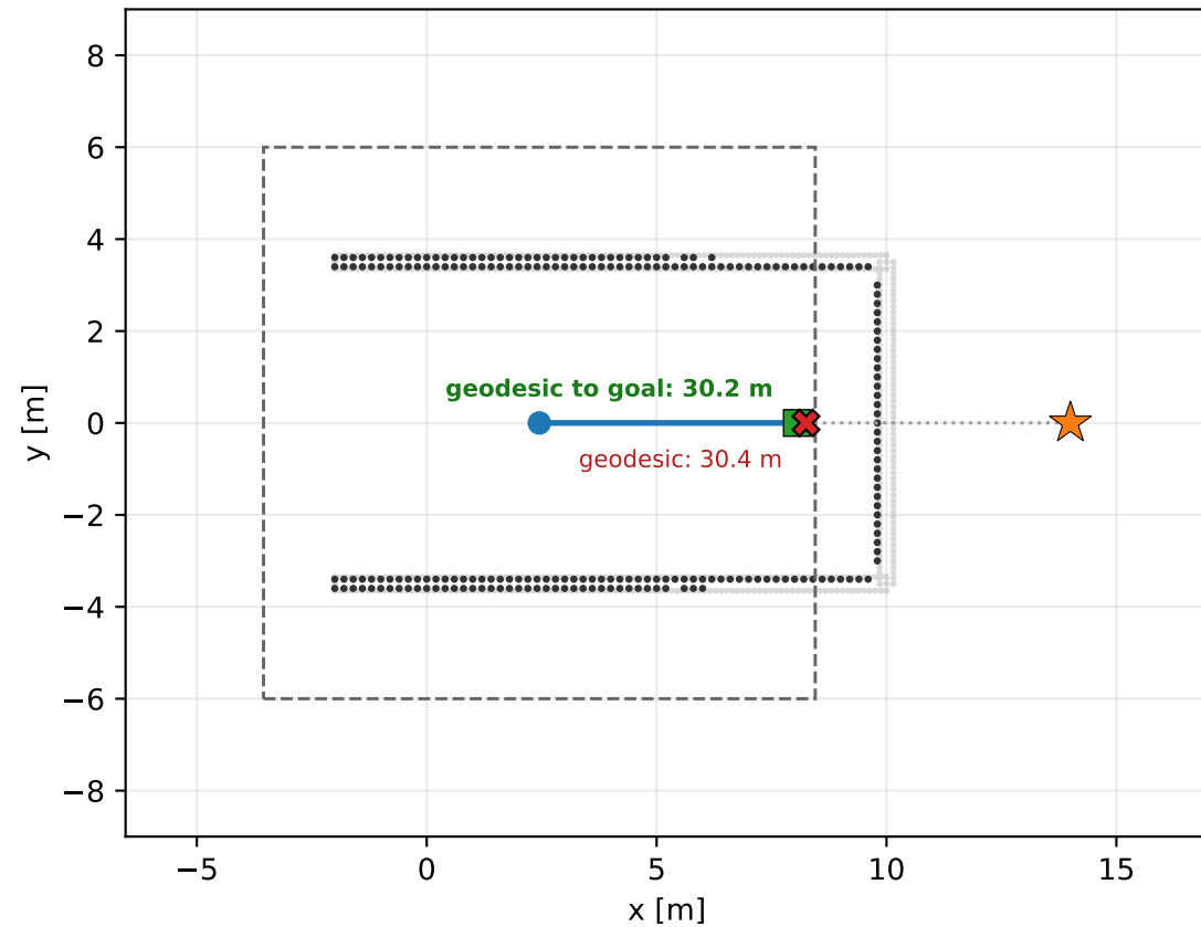
Baseline: projection along the ray to the goal
