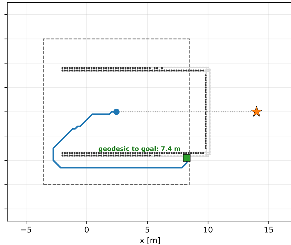
Deployed: arg min of the geodesic distance
