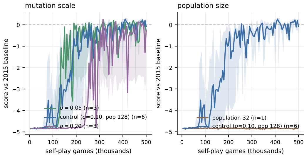
Figure 8: Mutation scale (left) and population size (right) against the control, median and inter-quartile band across seeds.
