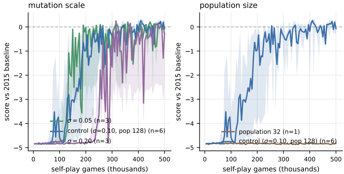
Figure 9: Mutation scale and population size against the control.
