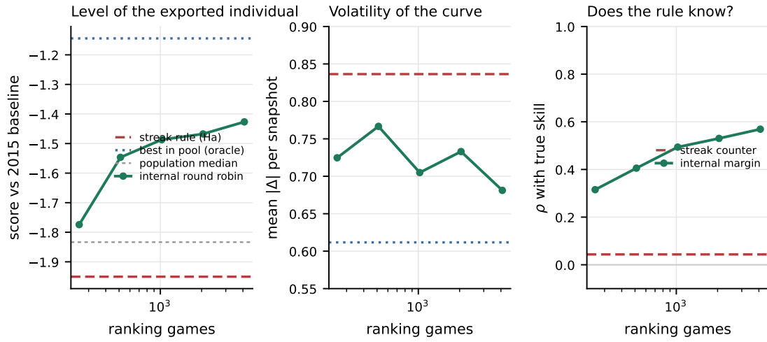
Figure 8: Promotion rules as a function of the games spent ranking.
