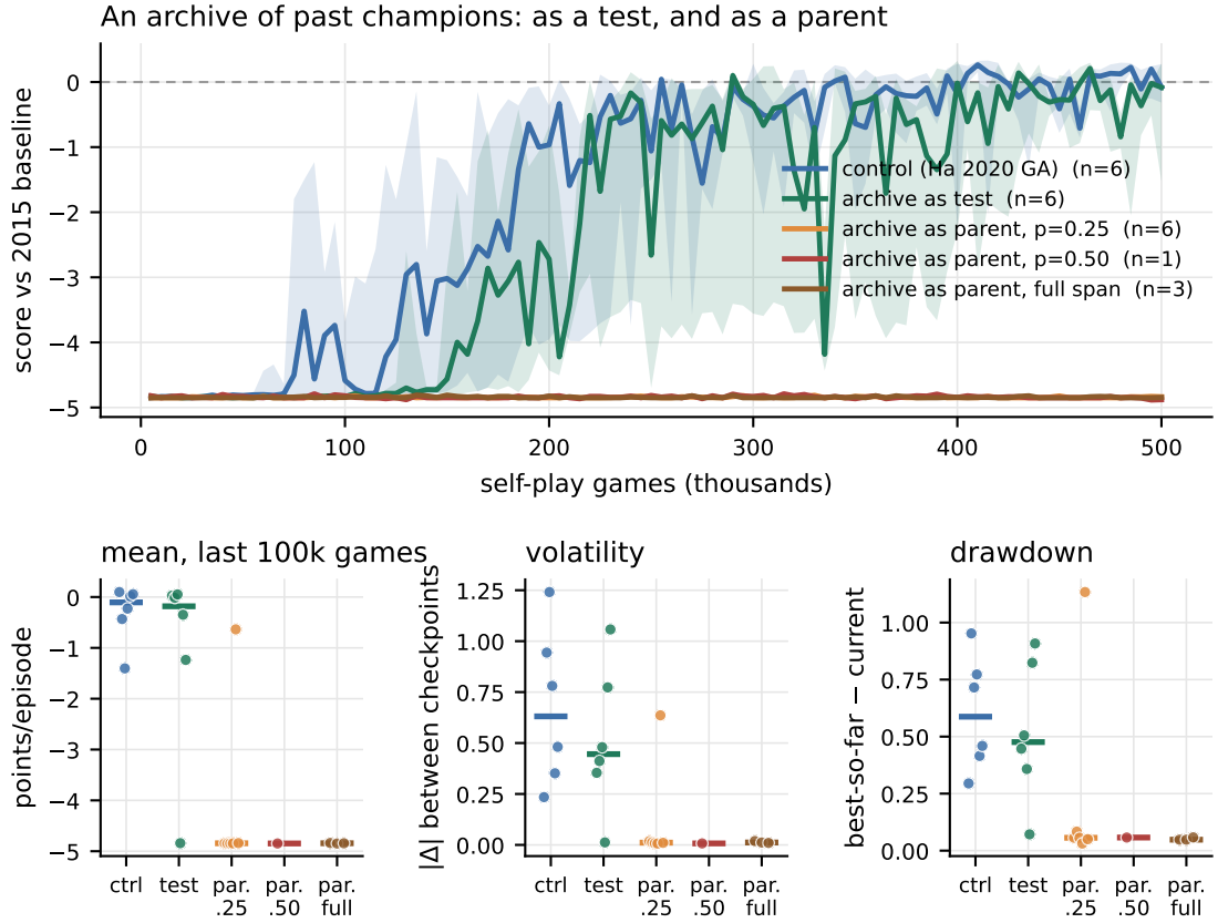
Figure 10: The archive conditions against the control. Bottom panels: ctrl, control; test, archive as test; par., archive as parent at the dose or span given in the legend.
