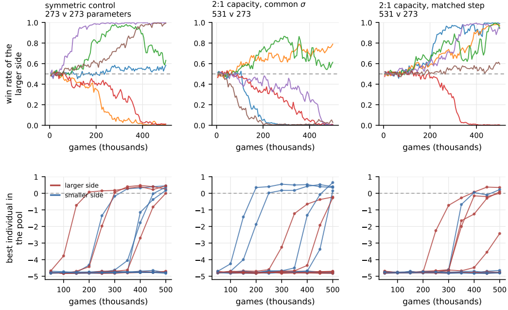
Figure 7: Two-population runs (exploratory, Section 4). Top: the larger side’s win rate in cross-population games, one line per seed. Bottom: the best member of each pool against the 2015 policy (red: larger side, blue: smaller).
