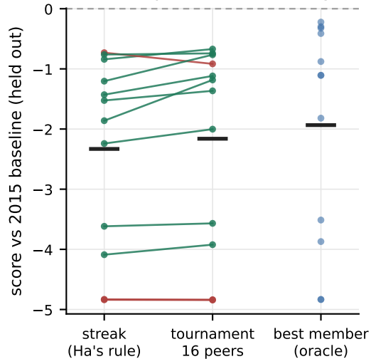
Slime Volleyball: 9 of 12 runs higher
