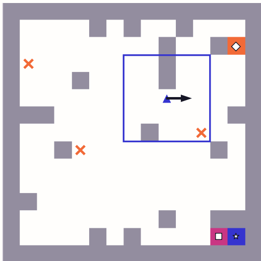
A Retrospective true world
