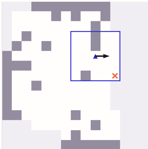
B Remembered terrain
