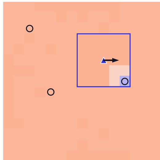
C Before-outcome forecast
