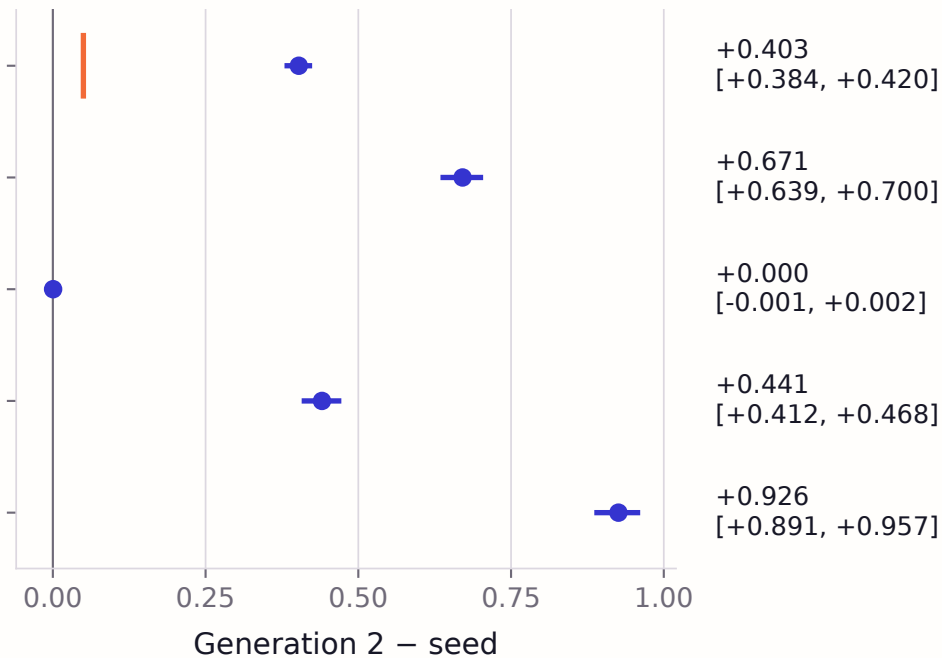
B Paired effects and 95% intervals
