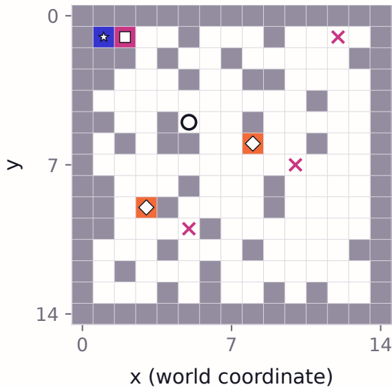
Last record · step 85 Hidden world (retrospective)
