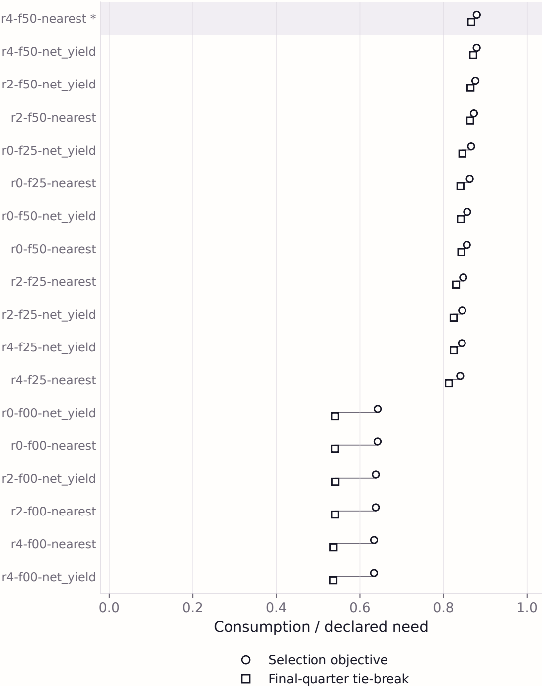
A Mean consumption and final-quarter consumption
