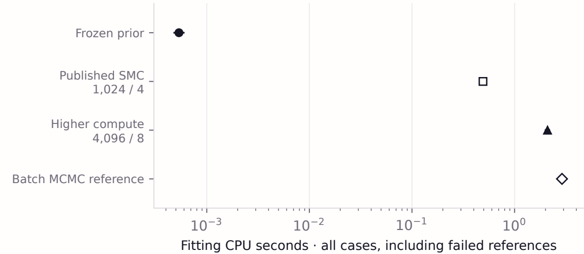
Prior-predictive control · n=128
