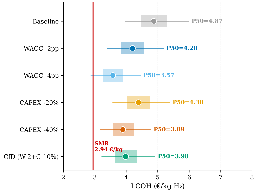
(a) LCOH distribution by policy scenario Box=P25-P75 | Line=P5-P95 | Dot=P50
