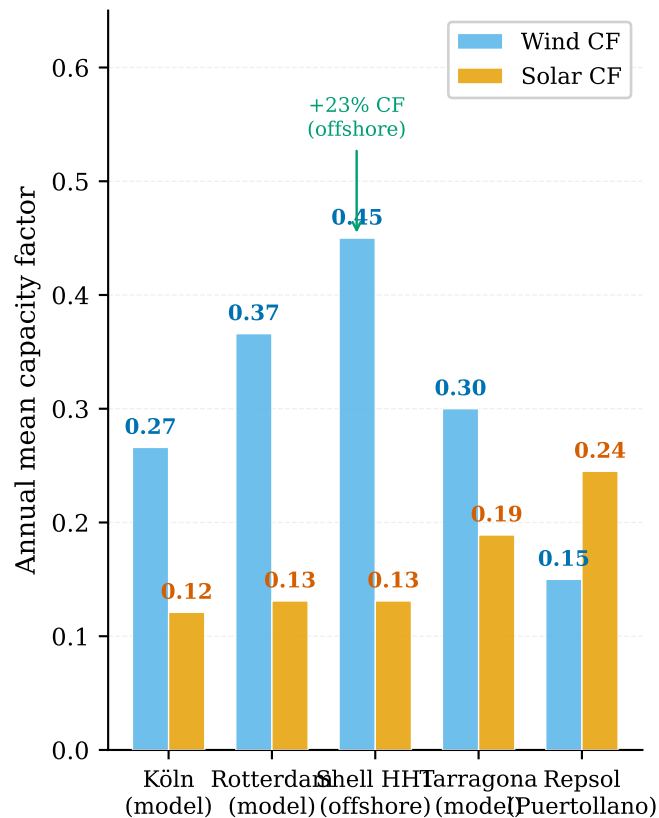
(b) Renewable CFs model vs real
