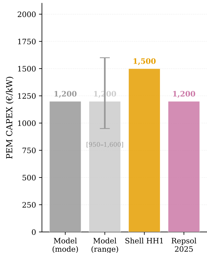
(a) PEM CAPEX model vs real
