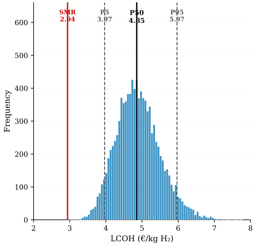
(a) LCOH distribution (N = 10,000)
