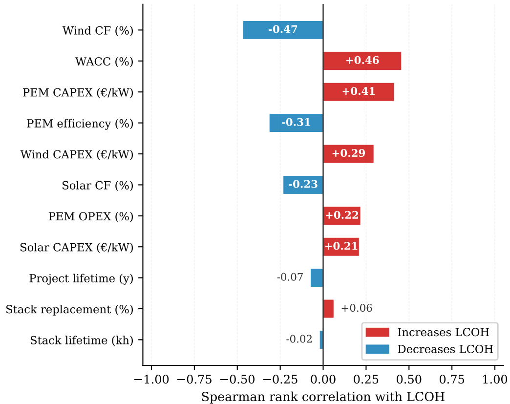
(b) Sensitivity — key cost drivers
