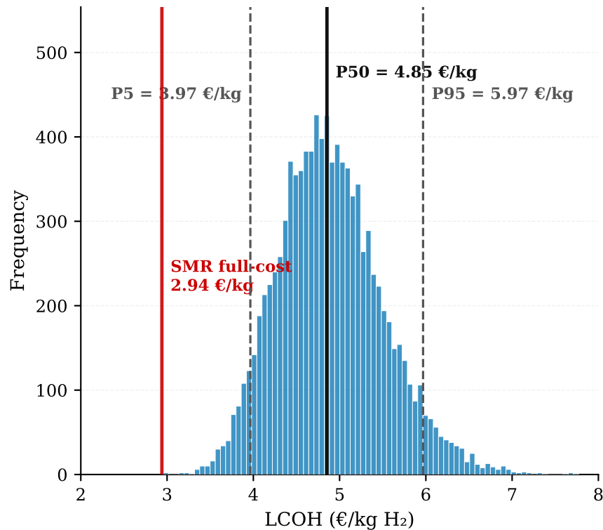
(a) LCOH distribution (N = 10,000) CF electrolyseur endogenous
