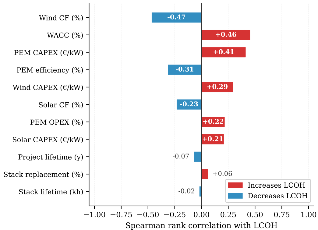
(b) Sensitivity — key cost drivers CF electrolyseur endogenous
