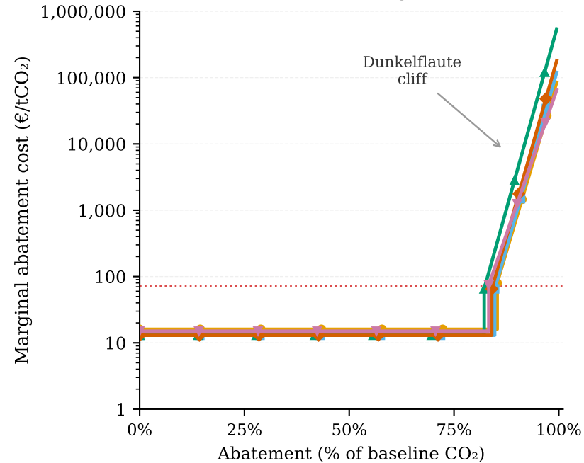
(a) Synthetic profiles no storage
