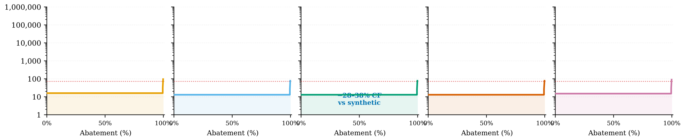
(c) Real profiles (OPSD 2019) — salt cavern
