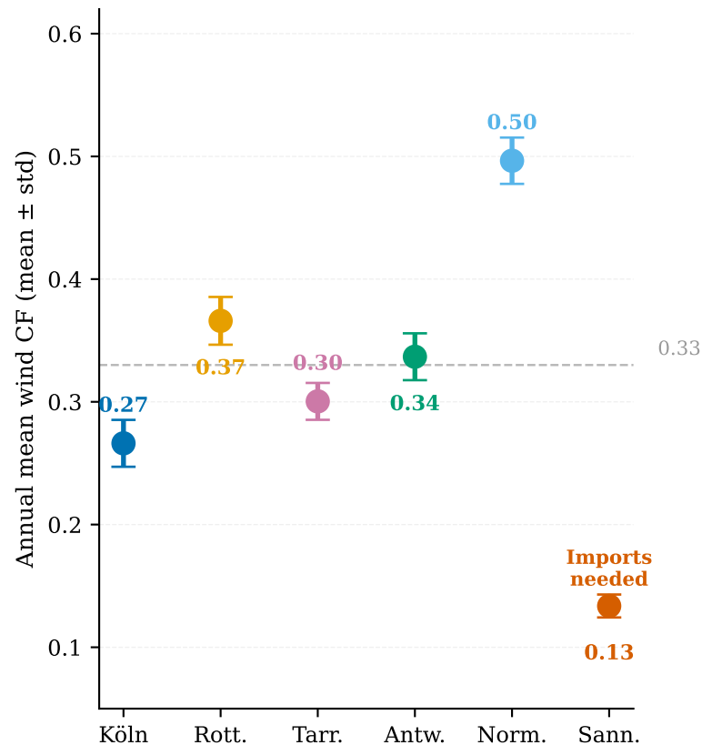
(b) Wind CF interannual variability 2019-2021
