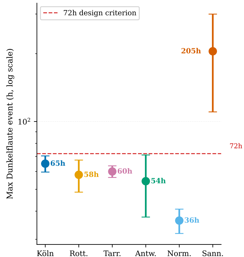
(c) Maximum low-wind event duration 2019-2021 (log scale)
