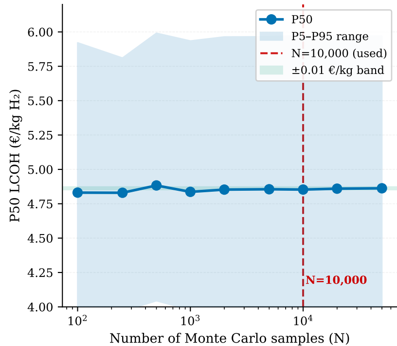
(a) Monte Carlo convergence — P50 N=10,000 within \pm 0.01 €/kg
