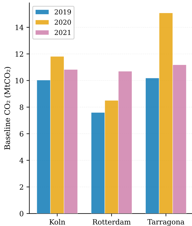
(b) CO 2 baseline by year
