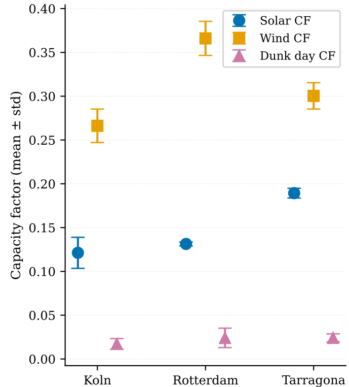
(c) Interannual variability 2019-2021
