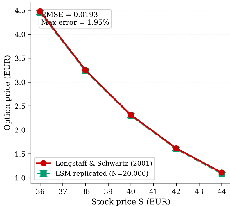
(b) American put: LSM vs L&S (2001) K=40 , T=1y , r=6\% , \sigma=20\%
