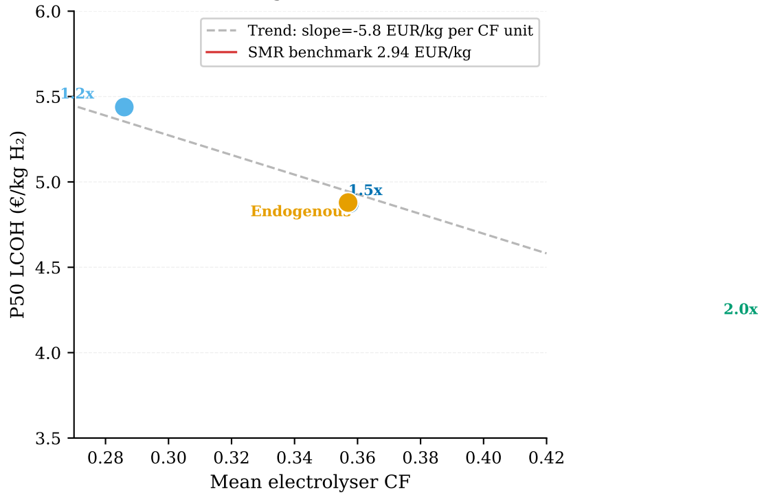
(b) Electrolyser CF vs P50 LCOH 1.5x oversized is IEA central estimate
