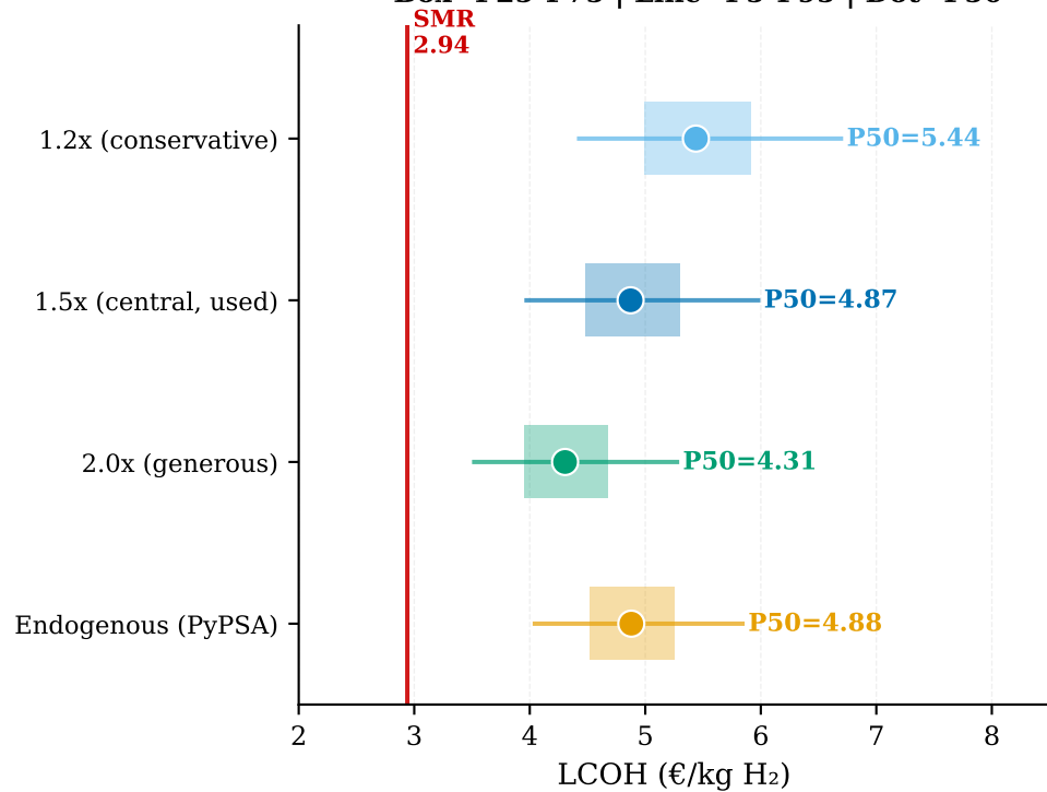
(a) LCOH sensitivity to oversized ratio Box=P25-P75 | Line=P5-P95 | Dot=P50
