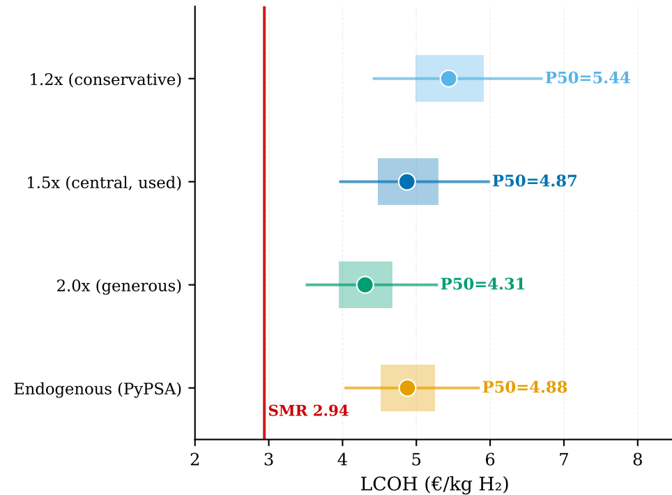
(a) LCOH sensitivity to oversizing ratio Box=P25-P75 | Line=P5-P95 | Dot=P50
