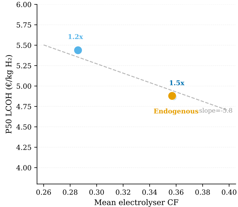
(b) Electrolyser CF vs P50 LCOH 1.5x oversizing: IEA GHR 2024 central
