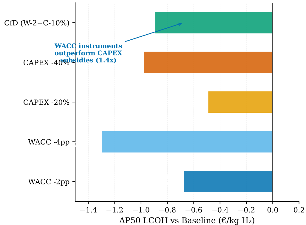
(b) Policy instrument effectiveness WACC -2pp vs CAPEX -20%: 1.4x more effective
