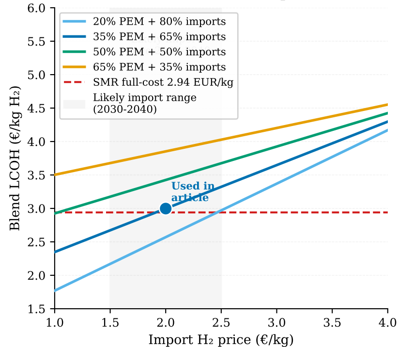
(a) Sannazzaro blend LCOH sensitivity PEM local + H 2 imports
