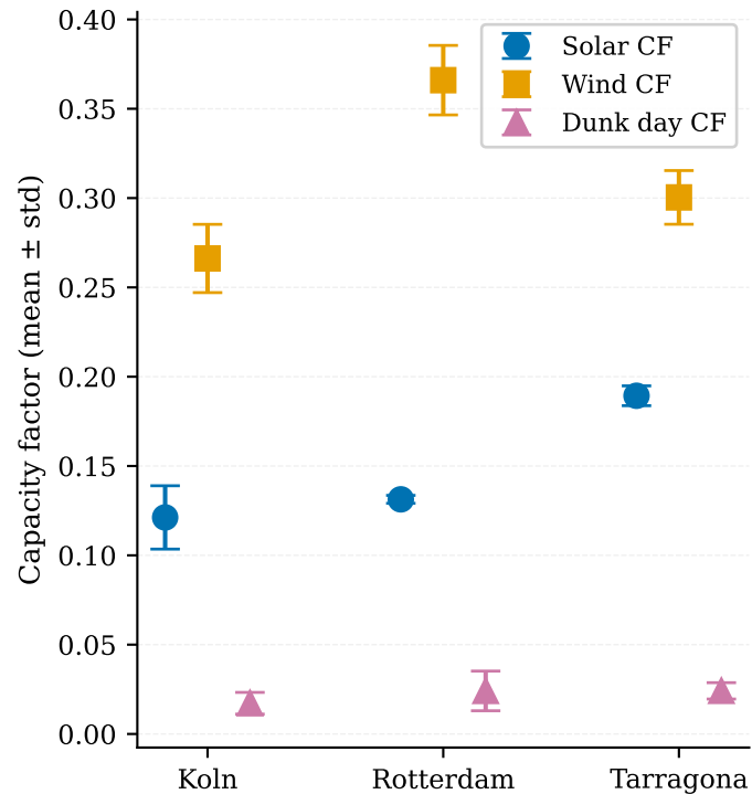
(c) Interannual variability 2019-2021
