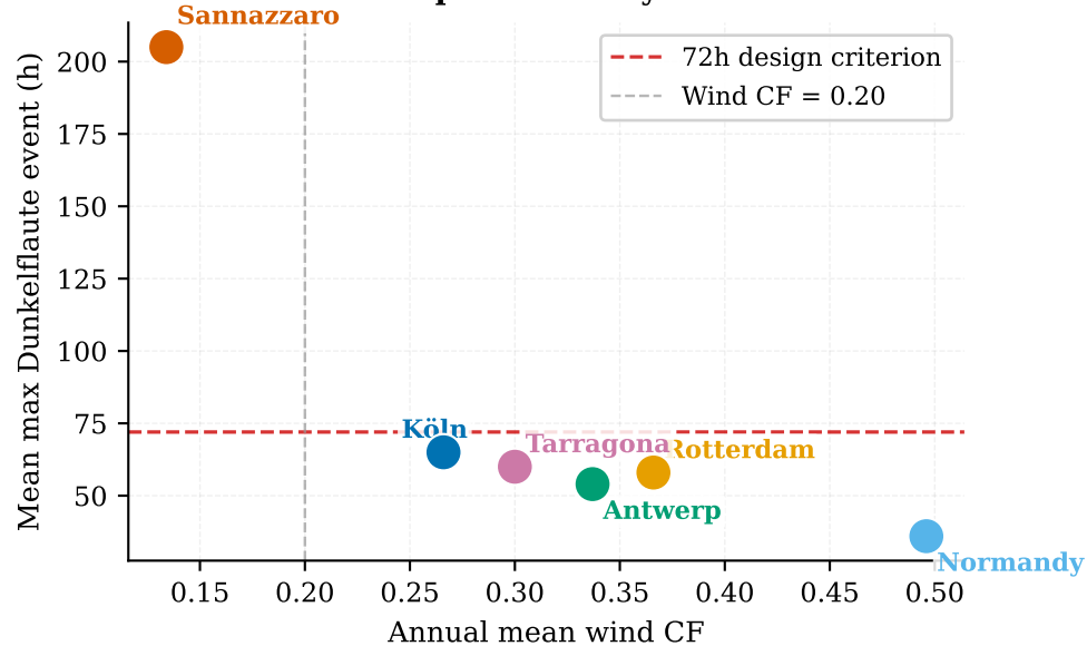
(c) Wind CF vs Dunkelflaute severity 6 European refinery locations
