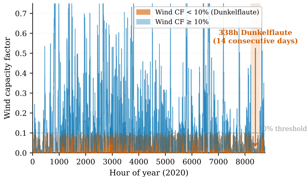
(a) Sannazzaro wind profile 2020 53-62% of hours below 10% CF
