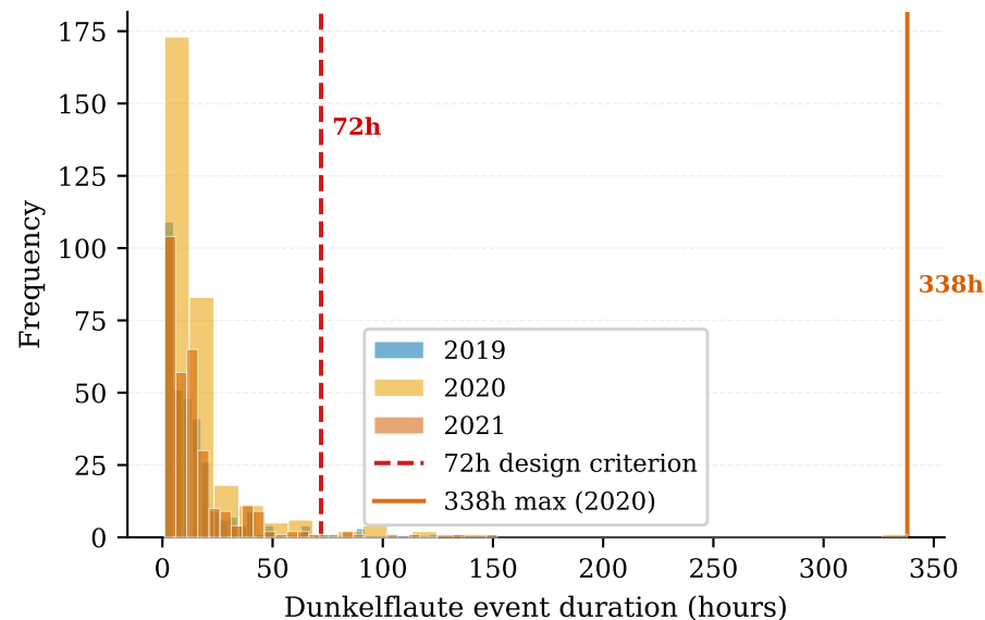
(b) Distribution of low-wind events (wind CF < 10%)
