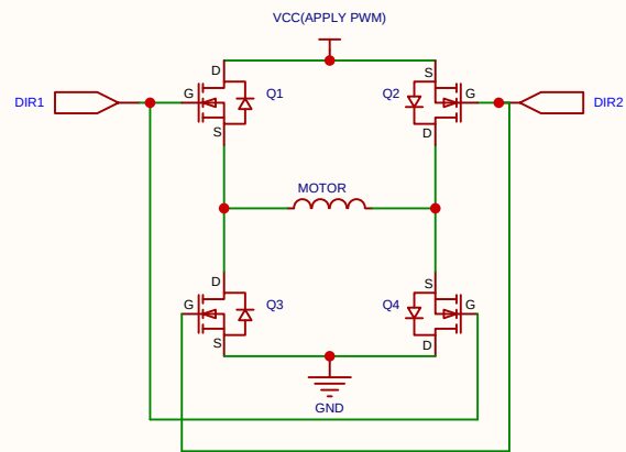
A H Bridge Motor Driver with PWM CONTROL and with N Mosfets
