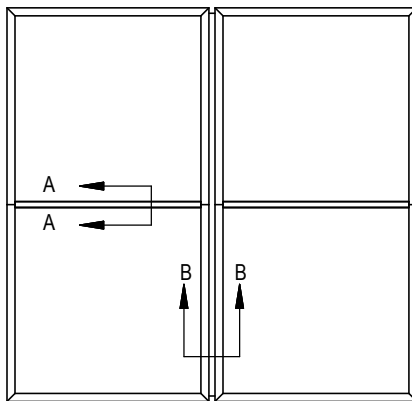
Both Dimensions Over 48" (1219mm) Sizes up to 96"x96" (2438mm x 2438mm) Mullions and Mounting Channel
