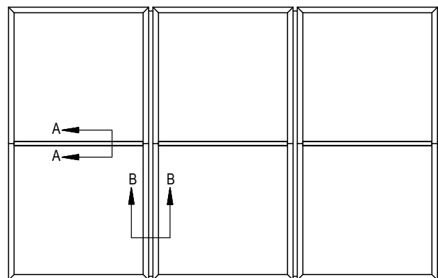
Both Dimensions Over 48" (1219mm) Sizes up to 144"x96" (3658mm x 2438mm) Mullions and Two Mounting Channels
