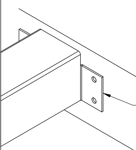
Both Dimensions Over 48" (1219mm) Sizes up to 96"x96" (2438mm x 2438mm) Mullions and Mounting Channel
