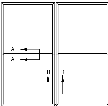
Both Dimensions Over 48" (1219mm) Sizes up to 96"x96" (2438mm x 2438mm) Mullions and Mounting Channel
