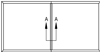
One dimension over 48" (1219mm) Sizes up to 96" x 48" (2438mm x 1219mm) Two Sections with Mullion
