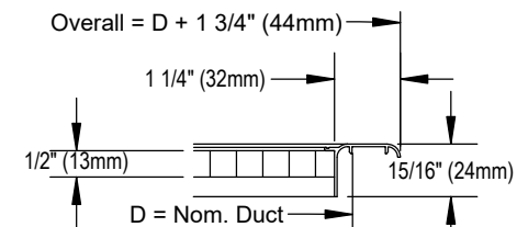
□ C - Curved Face Border (Surface Mount)
