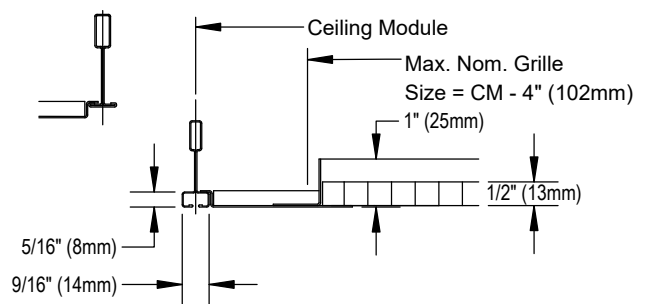
□ N - Narrow Flat Face Border (Surface Mount)
