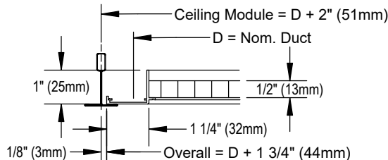
□ F - Flat Face Border (T-Bar Lay-in)
