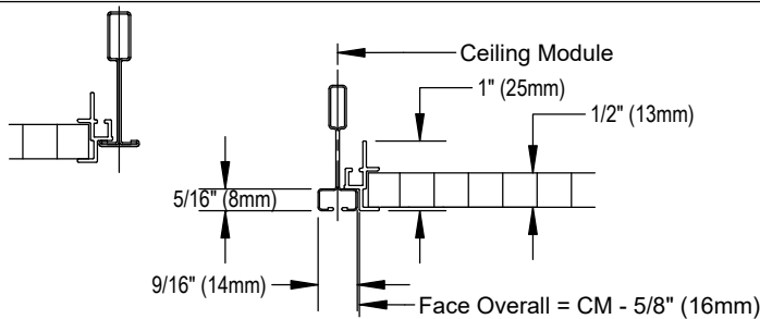
□ 17 - 9/16" Bolt Slot or Tegular T-Bar
