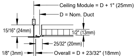
□ NF - Narrow Face Border (T-Bar Lay-in)
