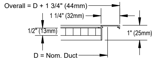
□ F - Flat Face Border (Surface Mount)
