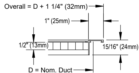
□ N - Narrow Flat Face Border (Surface Mount)
