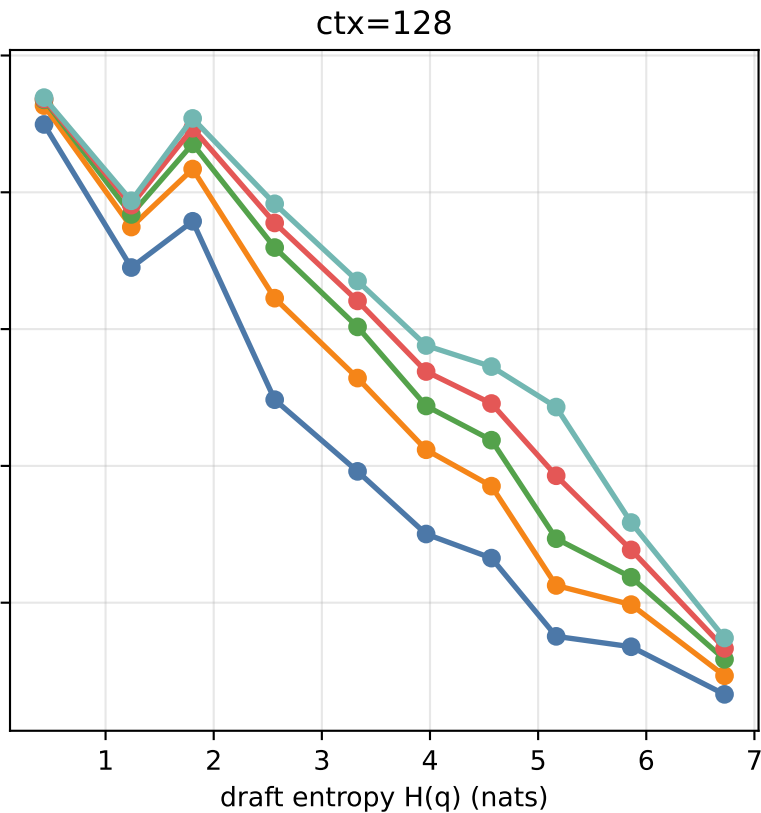
Greedy Accept@1.5 vs draft entropy
