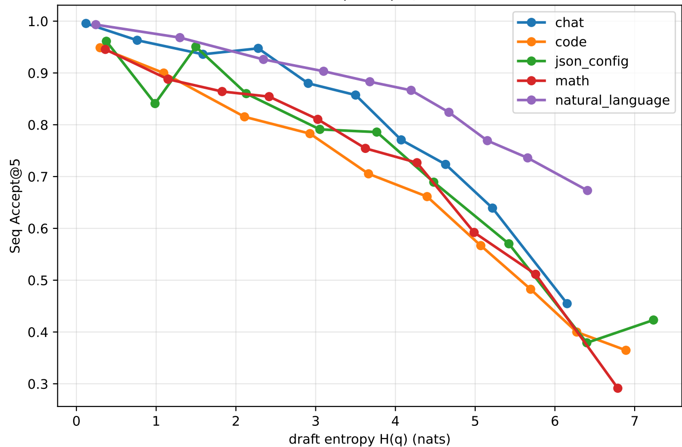
Per-source Seq Accept@5, ctx=256
