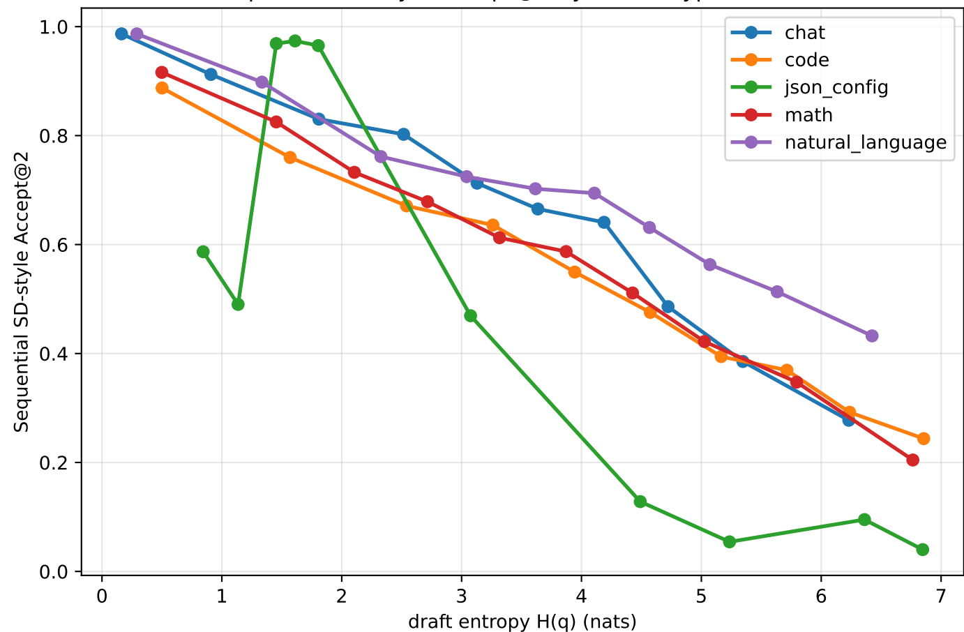
Sequential SD-style Accept@2 by source type, ctx=128
