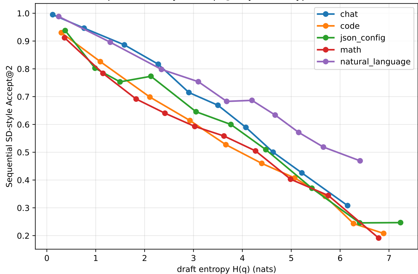
Sequential SD-style Accept@2 by source type, ctx=256
