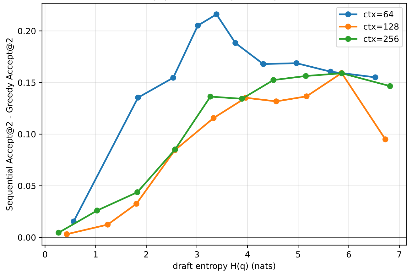
Performance gap between top-2 acceptance definitions
