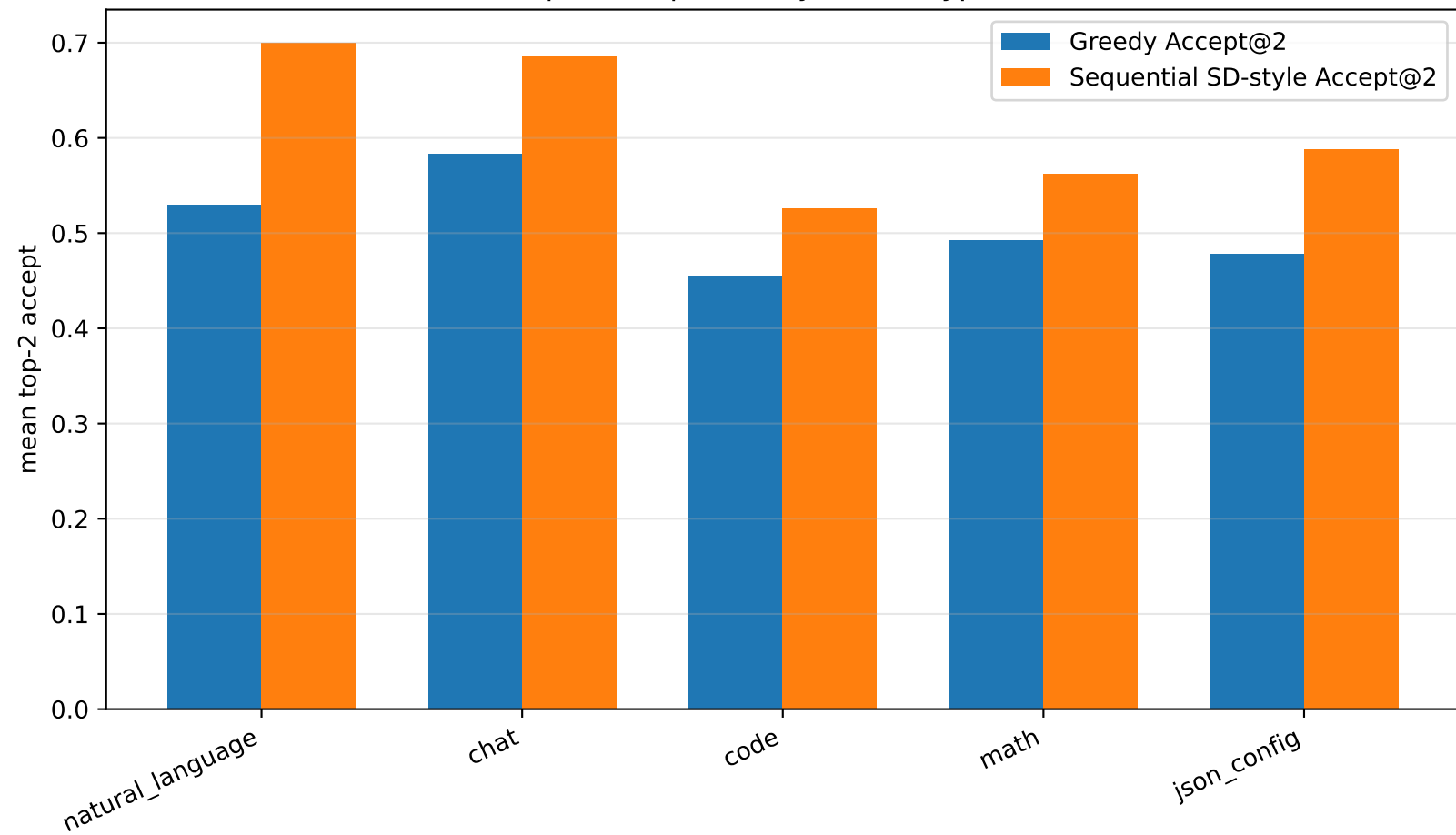
Mean top-2 acceptance by source type, ctx=256
