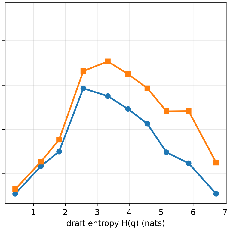
context length = 128
