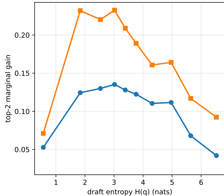
context length = 64
