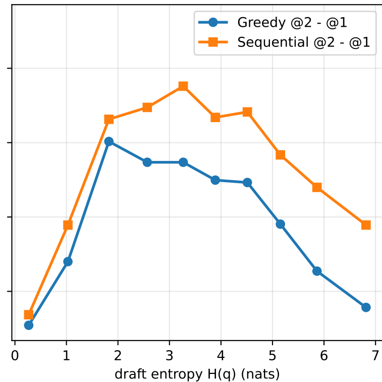
context length = 256
