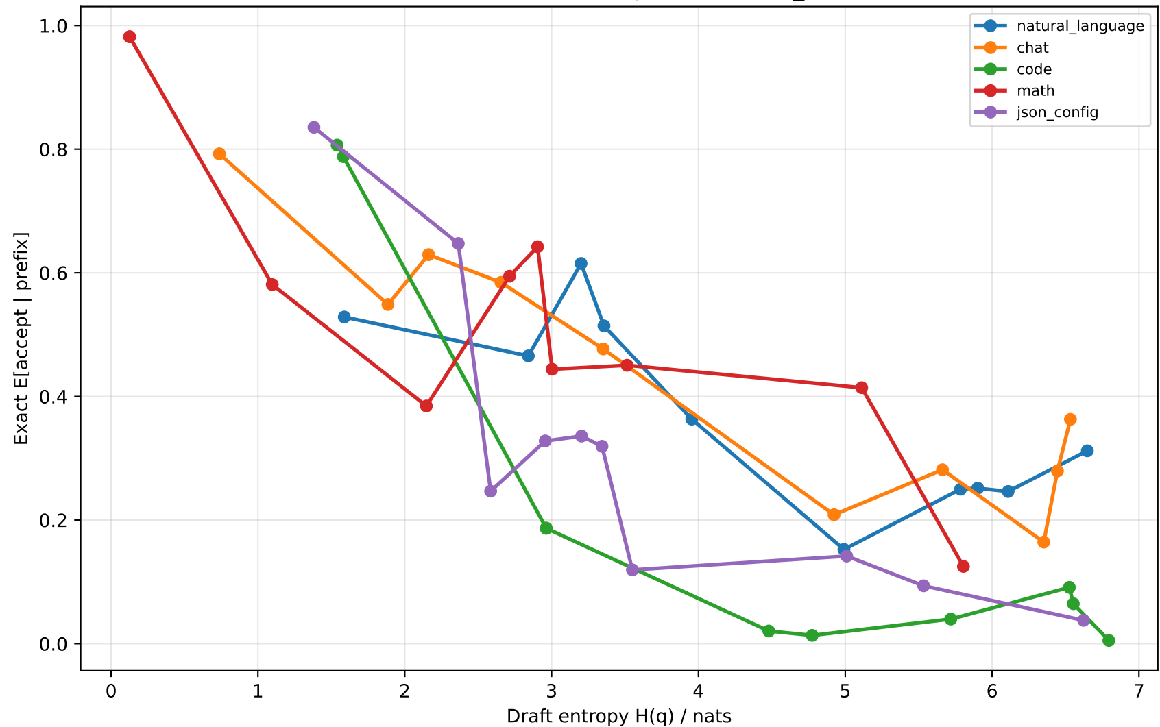
Per-source curves, natural prefix, context_len=128
