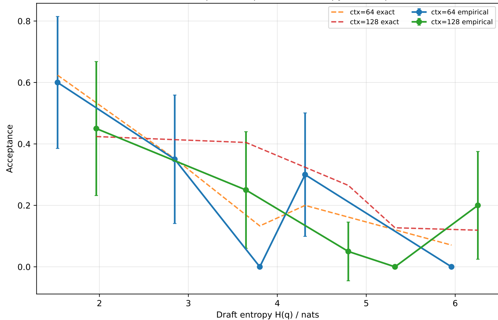
Balanced natural-prefix corpus: draft entropy vs acceptance
