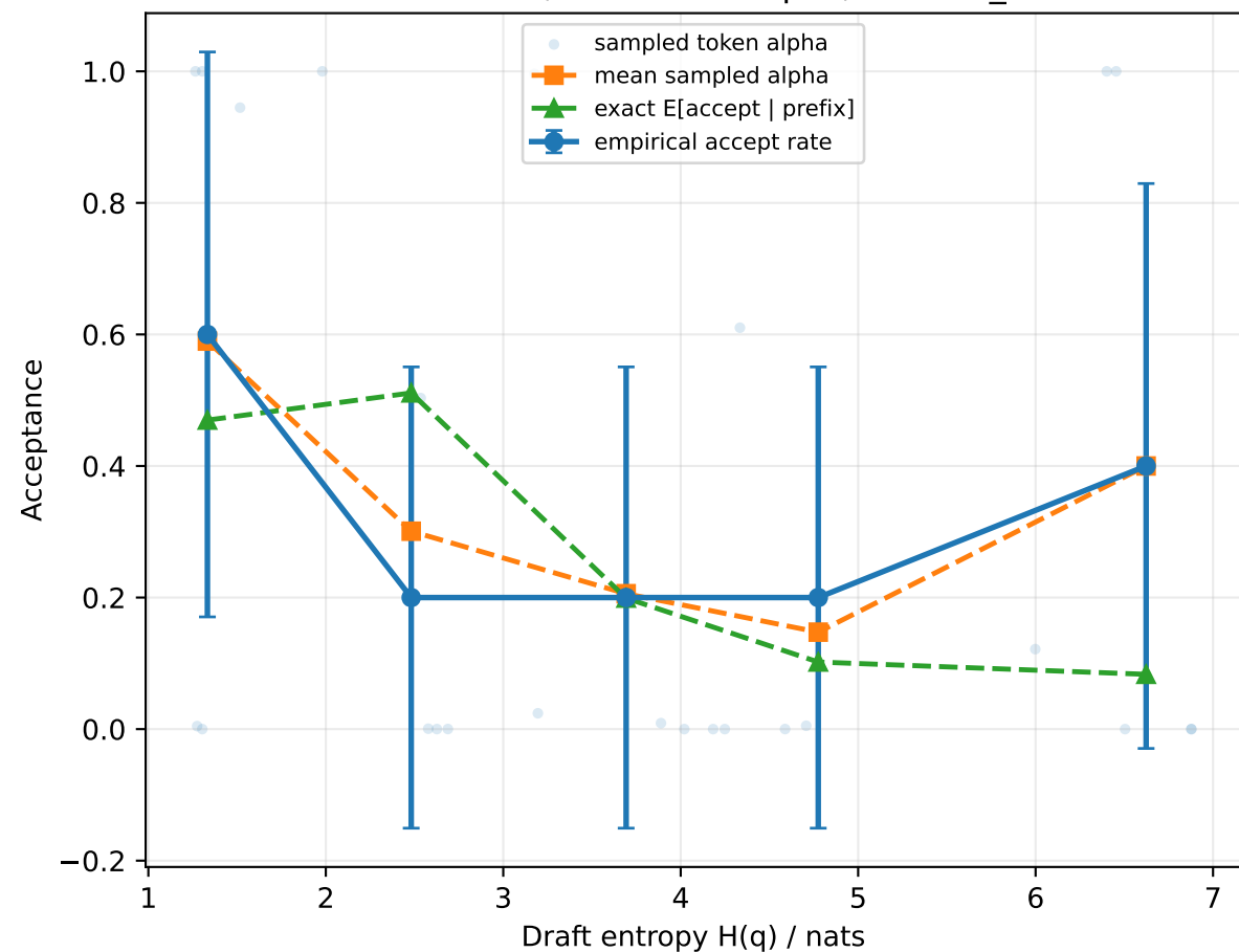
Detailed controls, balanced corpus, context_len=64
