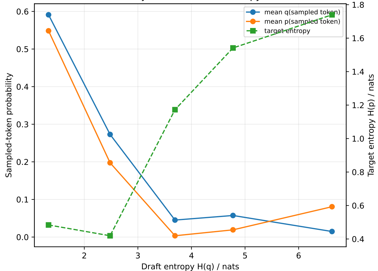
Probability controls across entropy bins
