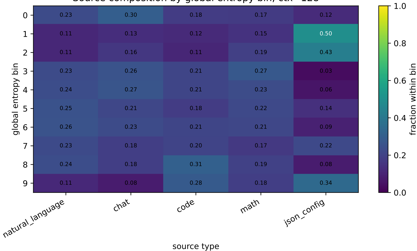
Source composition by global entropy bin, ctx=128
