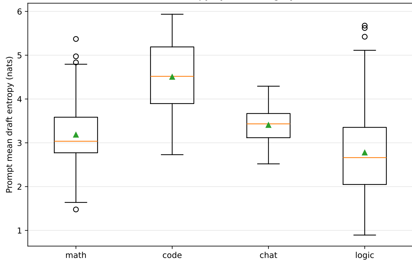
Draft entropy by task category
