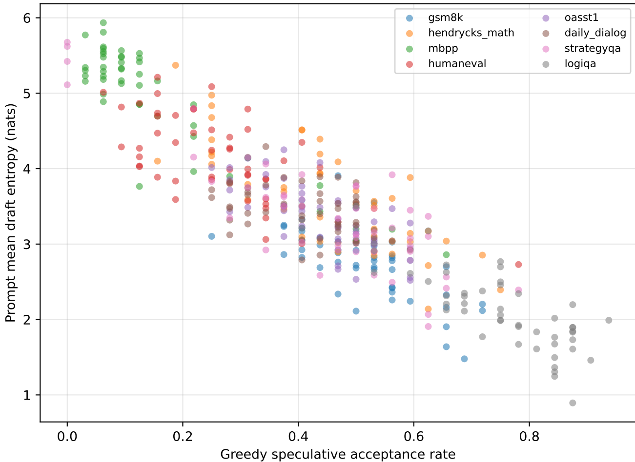
Draft entropy vs acceptance rate
