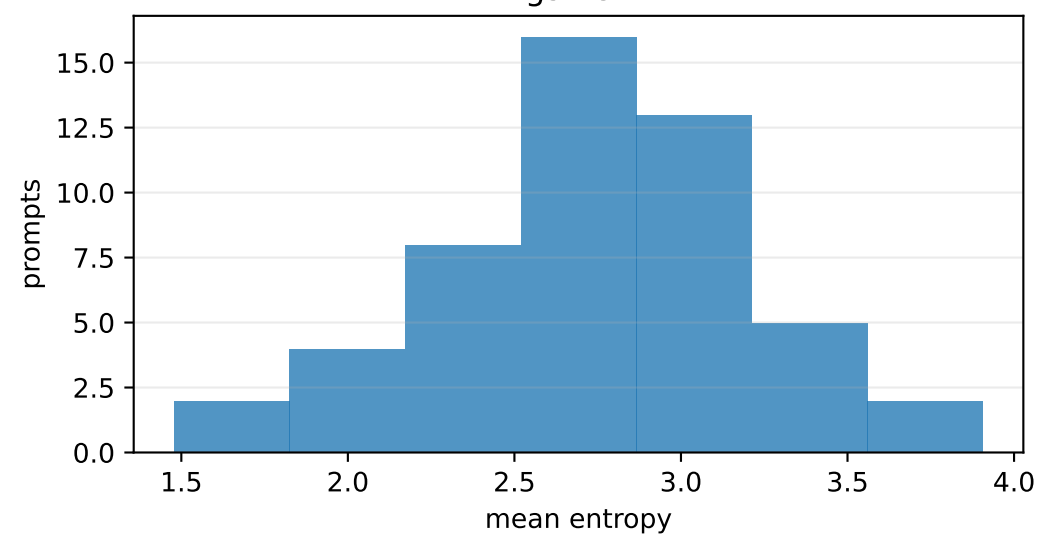
mbpp
