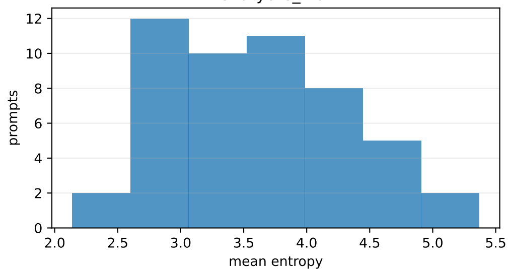
humaneval
