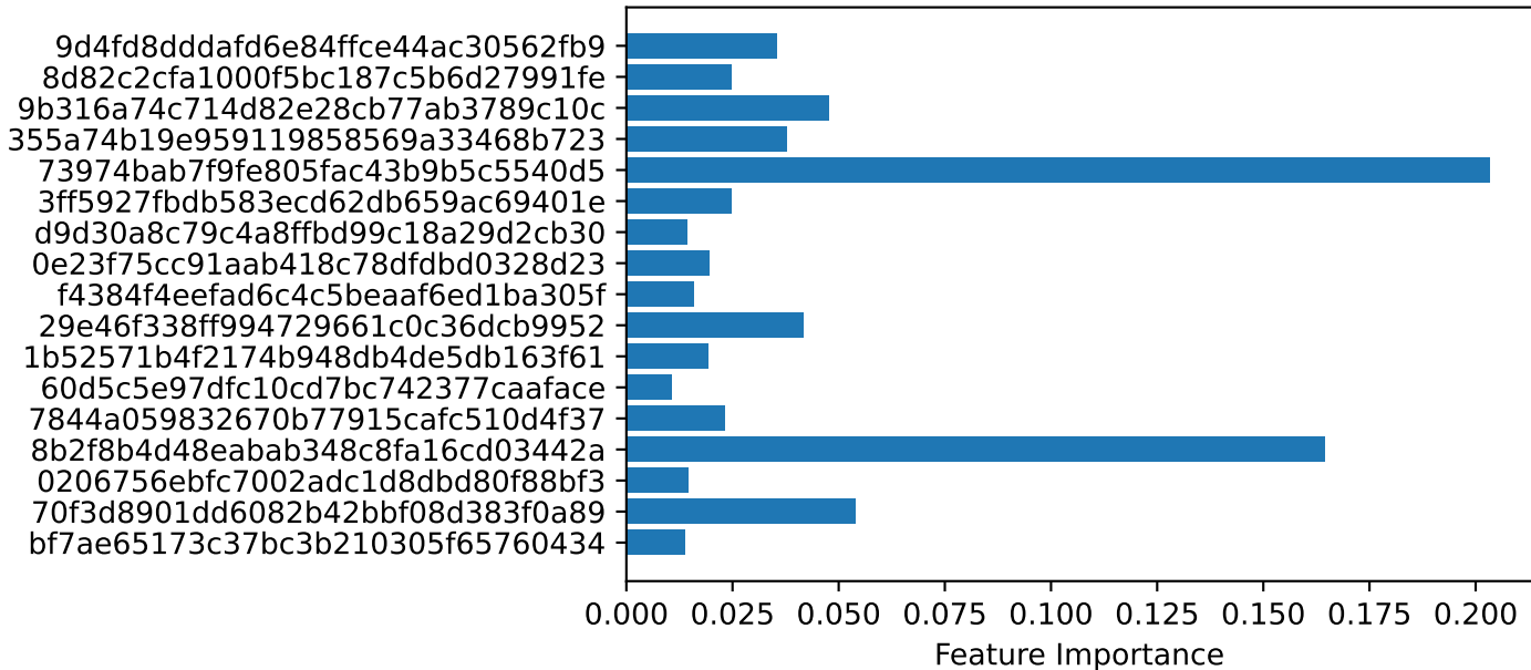
Feature Importance in Random Forest Classifier (above 1% importance)
