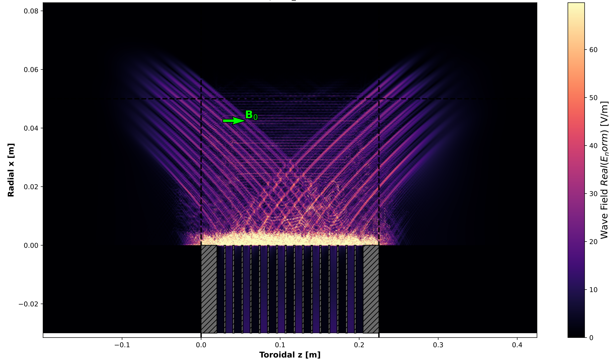
2D Map of E_{\text{norm}} (2D)
