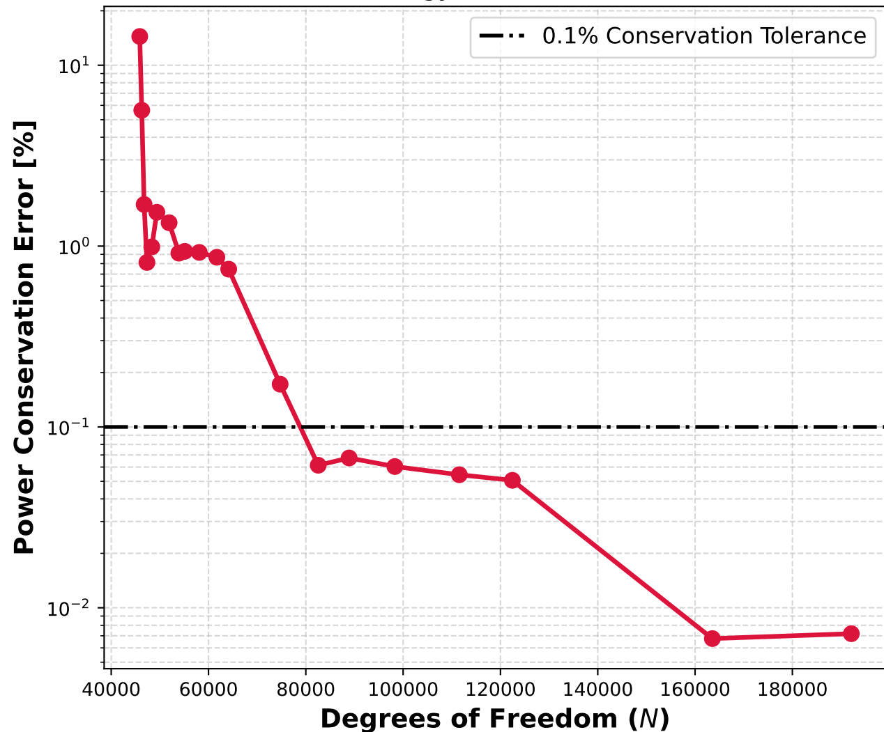
Global Energy Balance Verification
