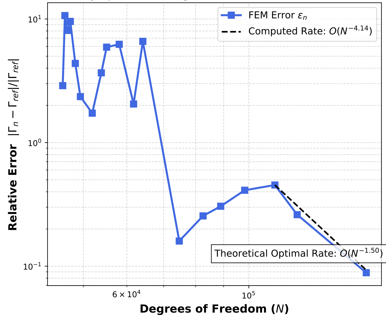
Asymptotic Convergence of Reflection Coefficient
