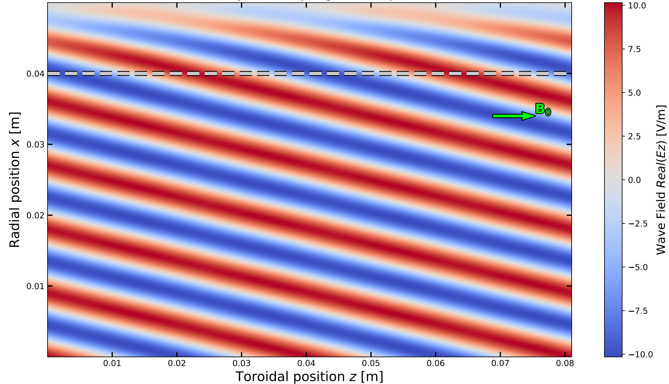
Lower Hybrid Coupling: E_z component
