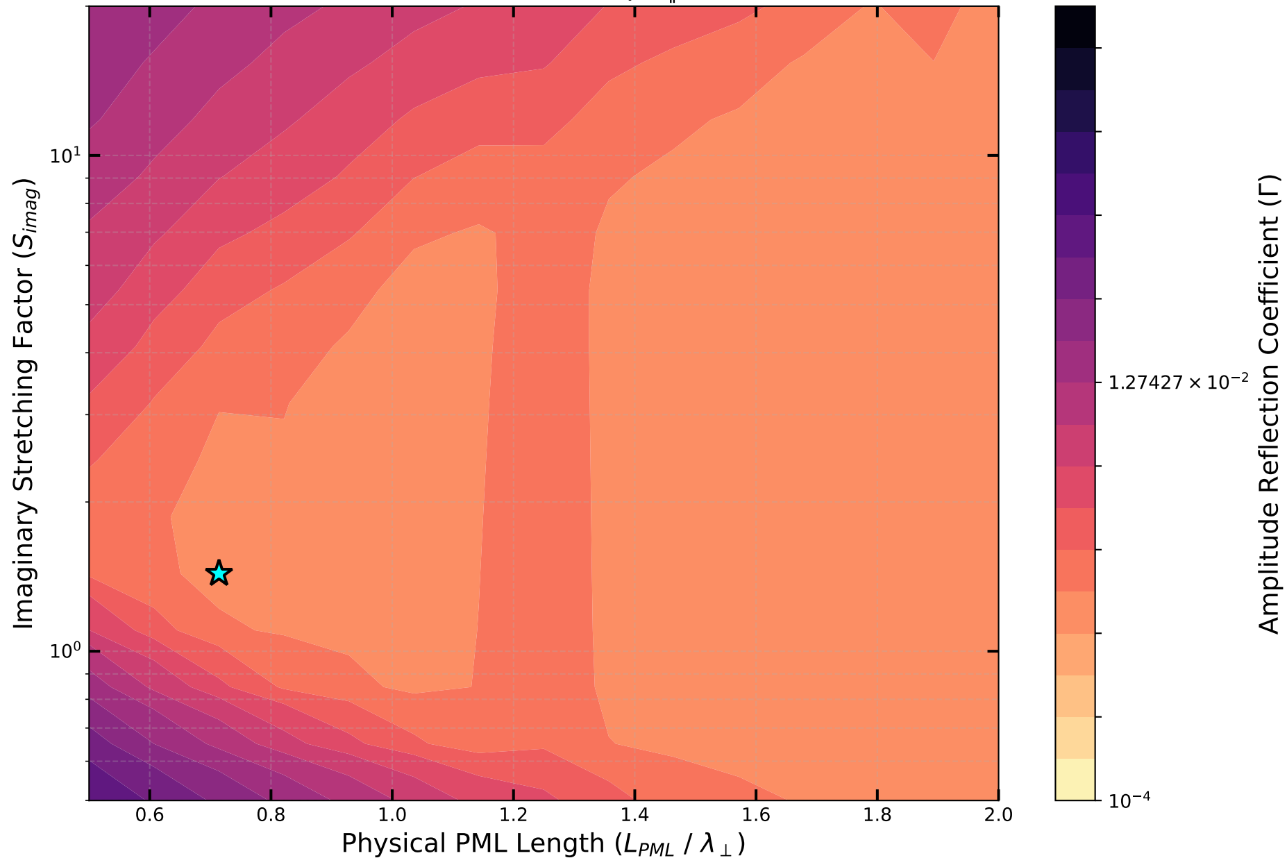
PML Efficiency Scan | n_{\parallel} = 2.0
