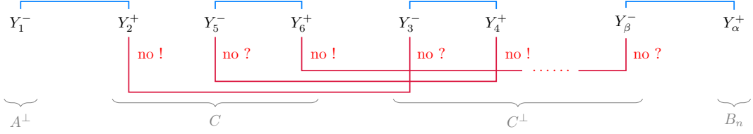
■ Figure 2 Alternating path p in the GOI projection graph \mathcal{G}_\mu in the proof of Proposition 14
